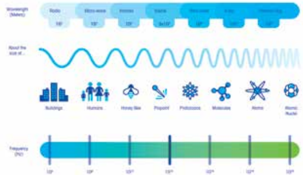
Figure 4: Electromagnetic Spectrum
