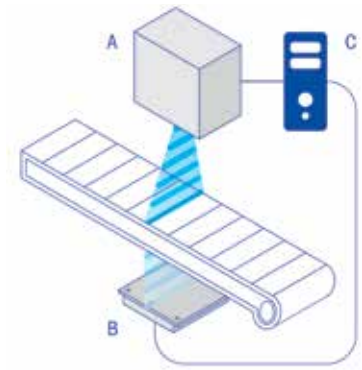
Figure 5: Components of an x-ray system
